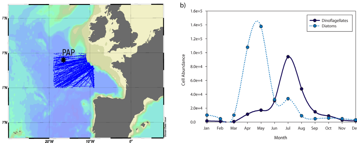
Figure 11. a) CPR towed routes between January 2001 and December 2007 in the waters surrounding the Porcupine Abyssal Plain (PAP) observatory. b) Average seasonal variation of diatom and dinoflagellate abundance (2001-2007).
